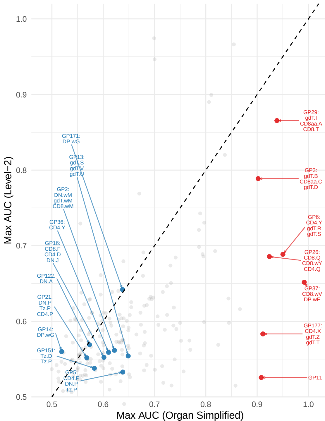
Max AUC: Organ vs Level-2 – organ-specific GPs
